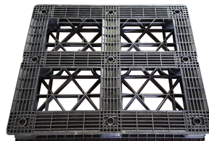
TDP PB Bottom View
